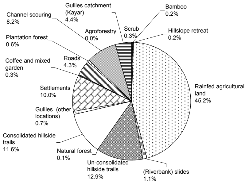
Fig. 3 Sediment sources in the upper Konto catchment.
